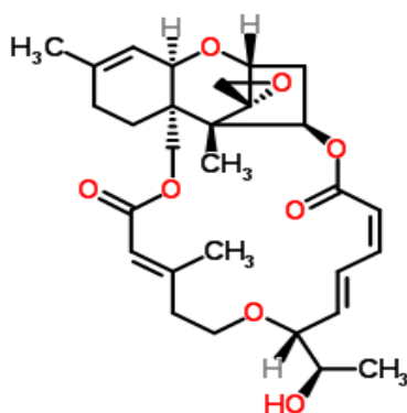
Figure 1. Roridin A
