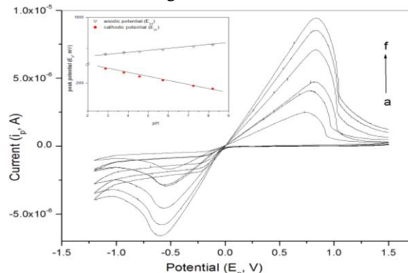
Fig. (4) , Cyclic voltammogram of 7.0 \mu\text{M} [\text{Ni}(\text{cpish})(\text{H}_2\text{O})\text{Cl}_2 \cdot 2\text{H}_2\text{O}] complex in 10% aqueous methanol (v/v) in universal buffer at scan rate 0.100 V/s, at different pH; a. 2.8, b. 8.2, c. 3.78, d. 4.56, e. 5.72 and f. 7.4, and the inserted figure shows the relation of the peak potential with the pH of the solution for both cathodic and anodic peaks.
