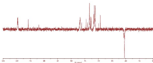
Fig15: ^{13}\text{C} -DEPT-135 Spectrum of Sweitenia mycophylla gum (10mg in 700 \mu\text{L} \text{D}_2\text{O} , 60 ^\circ\text{C} ) Referenced to TMSP
