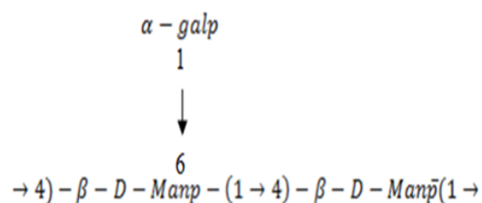
Fig 13: Skeleton of Chemical Structure of S.mycophylla
