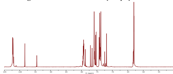
Fig 6: 13 C Spectrum of Swietenia microphylla gum (10mg in 700μL D 2 O, 60 o c) Referenced to TMS o P.
